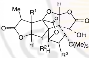
Ginkgolide structures
