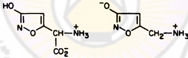
Ibotenic acid
