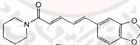
Piperine
