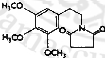
Mescaline succinimide
