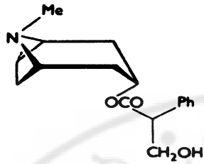
Hyoscyamine, Atropine
