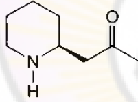
Pelletierine
