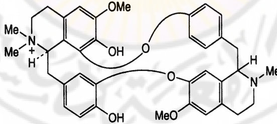
(+)-Tubocurarine
