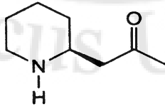
Pelletierine
