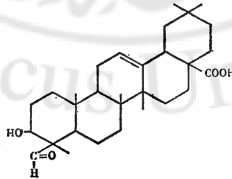
Gypsogenin
