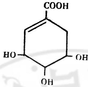
Shikimic acid
