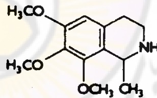
Anhalonine
